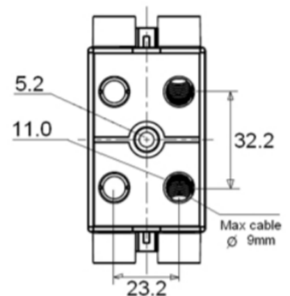
Back Wire Drilling
